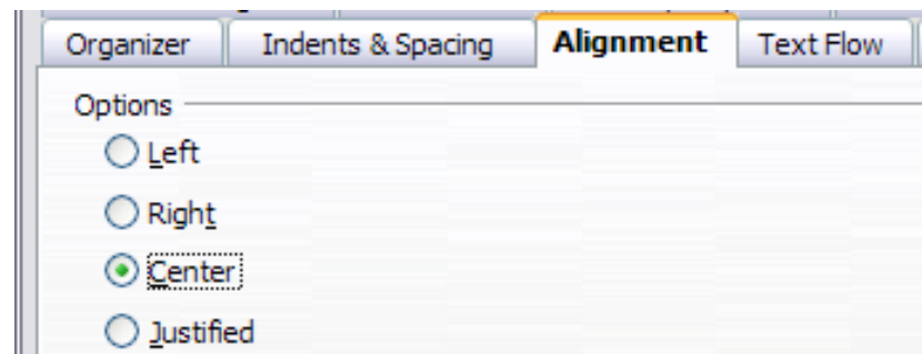
Figure 15: Center Heading 1
