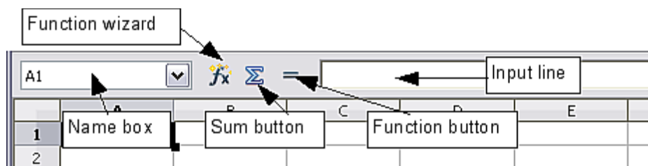
Figure 3. Formula Bar
