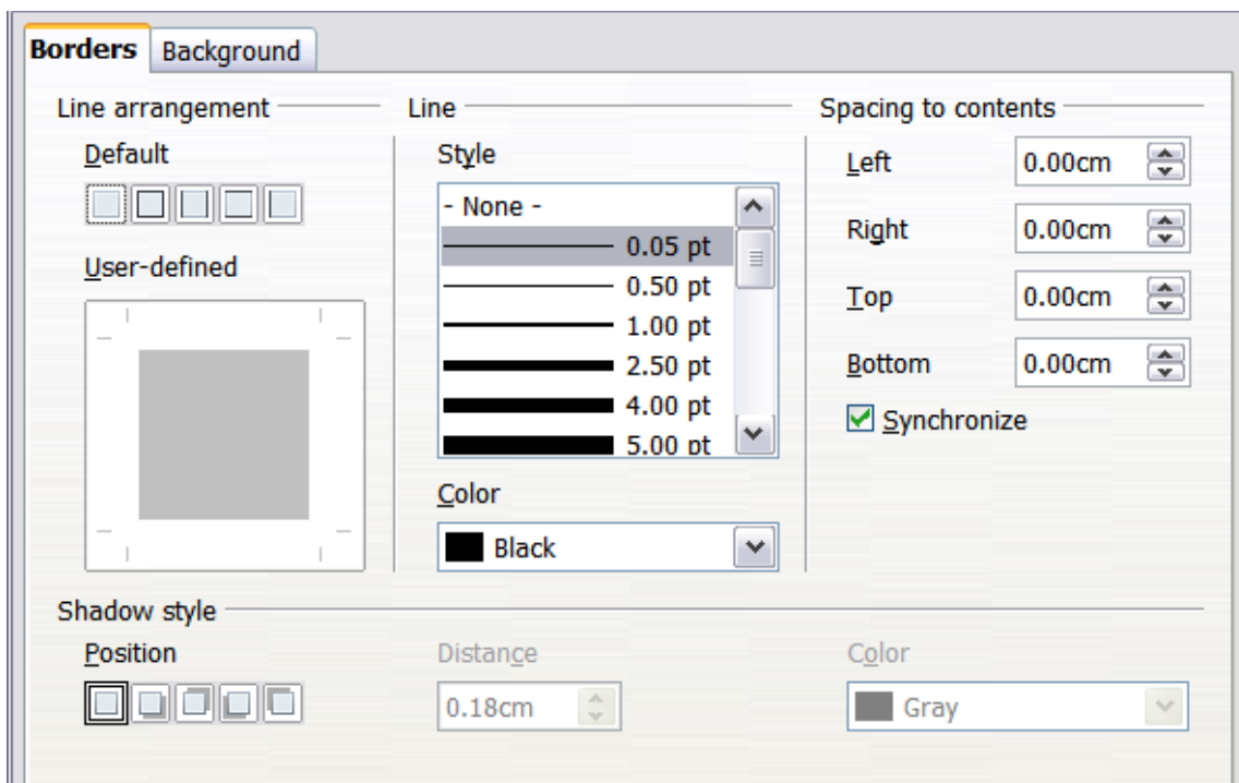
Figure 43: Header/Footer Border/Background
