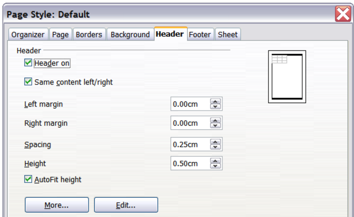
Figure 39: Header dialog
