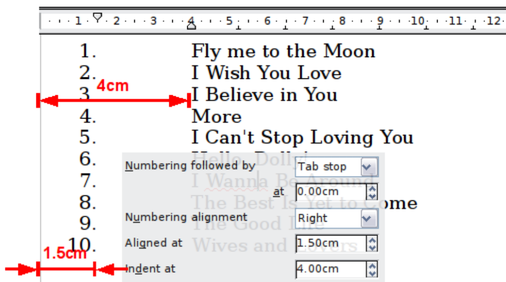
Figure 30: A numbered list of CD tracks highlighting the various elements
